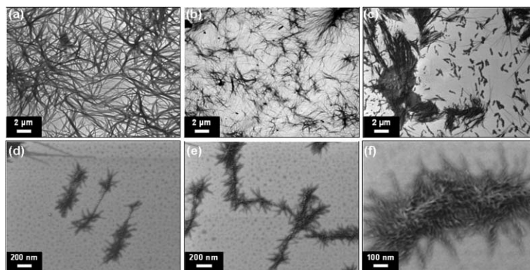
Fig. 3 Electron microscopy photographs: (a) TEM image of the toluene gel made of 2 (3 wt%), (b) TEM image of the toluene gel made of 2 (3 wt%) + 1b (molar ratio 2 : 1b = 10 : 1), (c–f) SEM images of the sample (b), (d–f) enlarged views of individual nanobrushes in (c).
