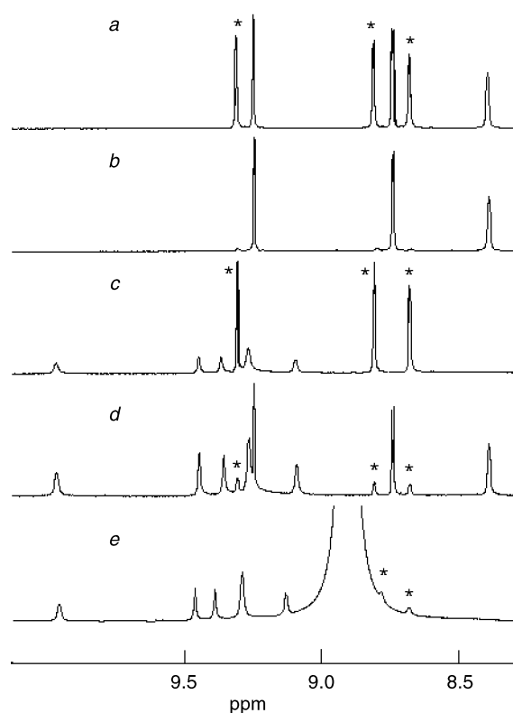
Fig. 13 500 MHz 1 H NMR spectra of (a) n -Bu 4 NVO 3 + PCA (4 equiv.); (b) ( n -Bu 4 N) + [V(O) 2 (pca) 2 ] – (1); (c) n -Bu 4 NVO 3 + PCA (4 equiv.) + H 2 O 2 (1 equiv.); (d) 1 + H 2 O 2 (1 equiv.); (e) 1 + H 2 O 2 (50 equiv.). Peaks indicated by asterisks are due to free PCA. Concentration of the vanadium species was 5.0 × 10 –3 mol dm –3 .
