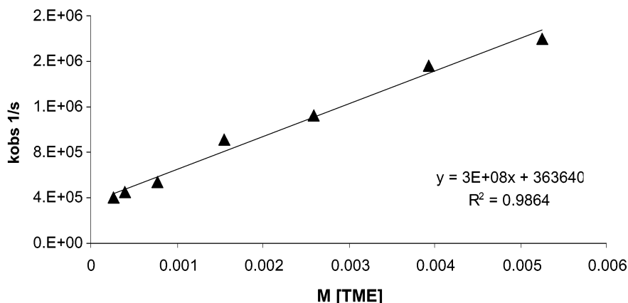
Figure 5. Plot of k_{\text{obs}} of the decay of the transient absorbing at 1142\text{ cm}^{-1} as a function of [\text{TME}] in heptane at ambient temperature.
