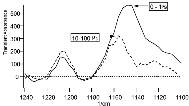
Figure 4. TRIR spectrum produced by LFP (266 nm) of 1 in heptane at ambient temperature (1 \mu\text{s}/\text{div} ).
