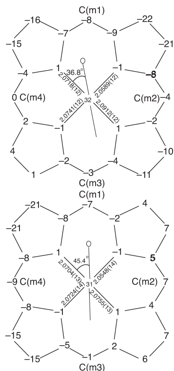
Figure 2. Formal diagrams of the porphyrinato cores. [Fe(TPP)-(Hdmpz)] (top) and [Fe(Tp-OCH 3 PP)(Hdmpz)] (bottom). Illustrated are the displacements of each atom from the mean plane of the four pyrrole nitrogen in units of 0.01 Å. Positive values of displacement are toward the imidazole ligand. The diagrams also show the orientation of the pyrazole ligand with respect to the atoms of the porphyrin core. The location of the methyl group at the \alpha -position of the coordinated nitrogen is represented by the circle.
