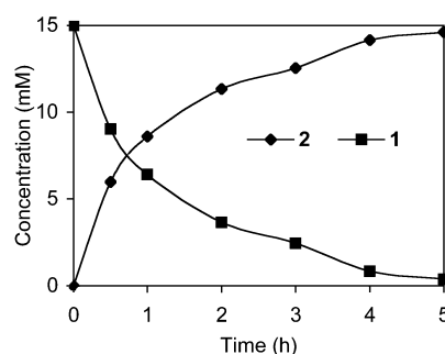
Fig. 1 Preparation of 2 by hydrolysis of 1 (15 mM) with frozen/thawed cells (10 g L -1 ) of Sphingomonas sp. HXN-200.
