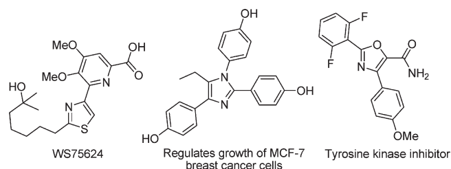
FIGURE 1. Pharmaceutically relevant azoles.
