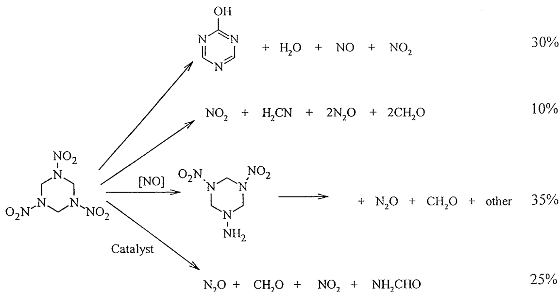
Figure 1. Decomposition pathway of RDX (ref 6).
