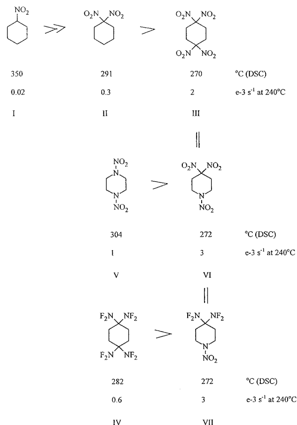
Figure 5. Thermal stability comparison of compounds studied.
