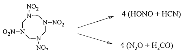
Figure 2. Decomposition pathway of HMX (ref 7).
