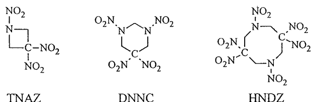
Figure 3. Structures of nitramines (ref 21).
