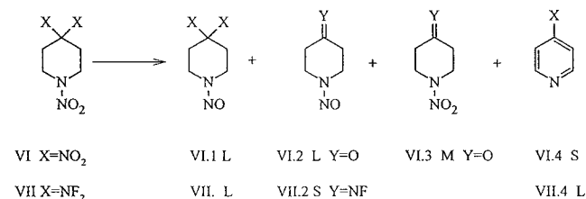
Figure 4. Decomposition products of nitramines VI and VII compared.
