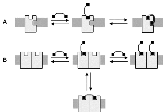
Figure 7. Bivalent ligand binding to (A) a GPCR with an accessory binding site or to (B) a GPCR dimer (according to Portoghesi et al. 35 ).
