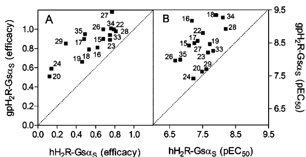
Figure 3. Efficacies ( E_{\max} ) and agonistic potencies of compounds 15–20, 22–24, 26–28, and 33–35 at hH_2R-Gs\alpha_S in comparison with gpH_2R-Gs\alpha_S as determined in the steady-state GTPase assay. The dotted lines represent the line of identity. (A) Plot of efficacies at gpH_2R-Gs\alpha_S vs hH_2R-Gs\alpha_S . (B) Plot of pEC_{50} at gpH_2R-Gs\alpha_S vs hH_2R-Gs\alpha_S .
