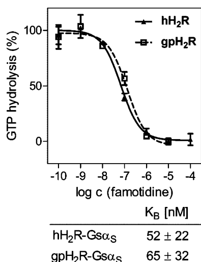
Figure 4. Concentration-dependent inhibition of GTP hydrolysis by famotidine using 33 as the H_2R agonist at 10 and 1 nM at the hH_2R-Gs\alpha_S (solid line) and the gpH_2R-Gs\alpha_S fusion proteins (dashed line), respectively. Data points are the mean of a representative experiment performed in duplicate.
