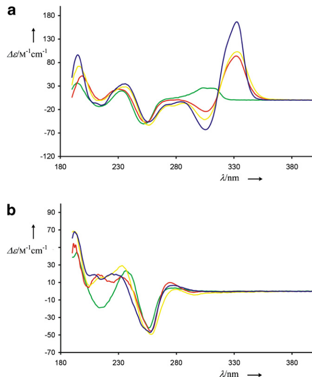
Fig. 3. CD spectra of the receptors (a) 1d (green) and (b) 1c (green) with \text{Ni}(\text{NO}_3)_2 (red), \text{Cu}(\text{CF}_3\text{SO}_3)_2 (yellow) and \text{Zn}(\text{CF}_3\text{SO}_3)_2 (blue) in \text{CH}_3\text{CN} .
