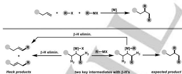
Scheme 1. Alkene 1,2-dicarbofunctionalization and complications by \beta -H elimination
