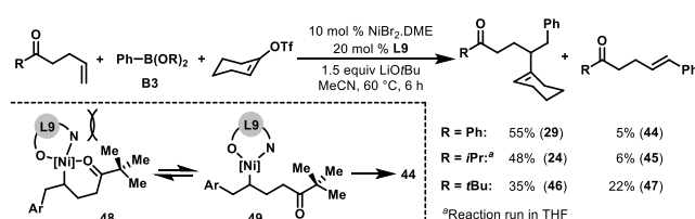
Scheme 4. Carbonyl steric effect
