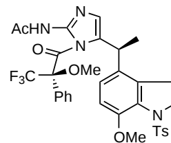
21 ( R )-MTPA derivative single peak at 1338.10 Hz
