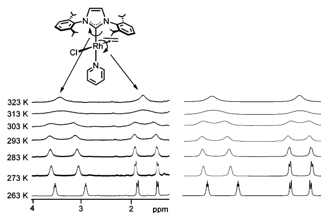
Figure 2. Variable-temperature ^1\text{H} NMR spectra of \text{RhCl(IPr)}(\text{pyridine})(\eta^2\text{-ethylene}) (4) in \text{CD}_2\text{Cl}_2 showing the coalescence of the CH–isopropyl and ethylene resonances: experimental (left) and calculated (right).
