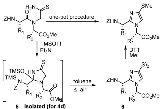
Scheme 2. One-Pot Procedure via a Silylated Intermediate
