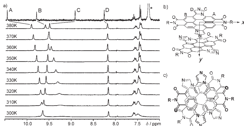
Figure 3. a) ^1\text{H} NMR spectrum (400 MHz) of 3 in \text{CDCl}_3 (top), and temperature-dependent ^1\text{H} NMR spectra of 3 recorded at 300 MHz in [\text{D}_6]\text{DMSO} . Side view (b) and top view (c) models for the aggregation behavior of 3 .
