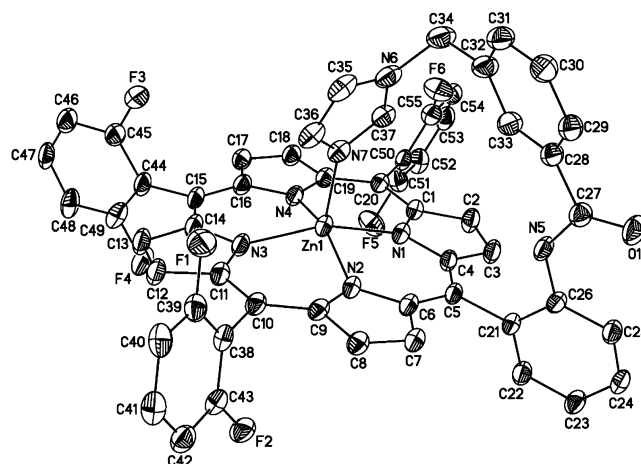
Figure 4. Molecular structure of [Zn(To-F 2 PP-BzIM)] showing IM bound to Zn(II) where the Zn ion is displaced from the porphyrin plane by 0.5 Å. Two CH 2 Cl 2 solvent molecules are present per unit cell and have been omitted, along with all hydrogen atoms, for clarity. Selected bond lengths are reported in Table 2. A complete list of all distances and angles is provided in the Supporting Information.
