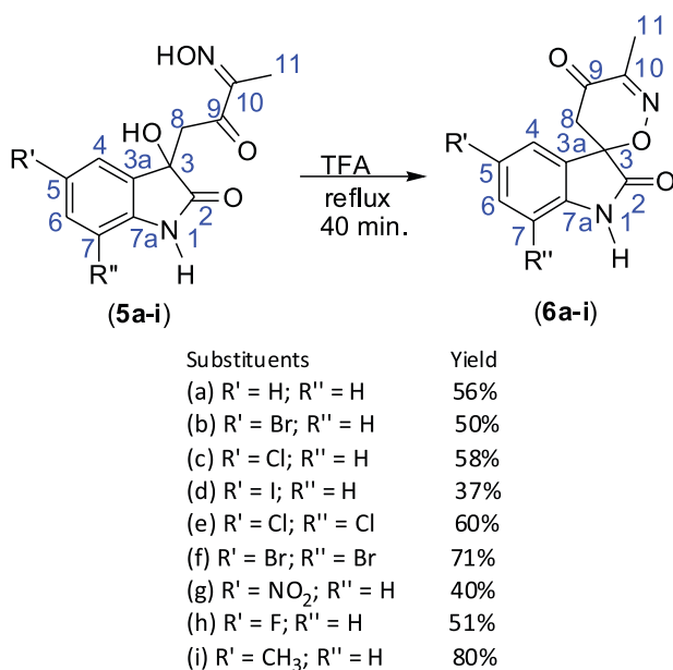
Scheme 1. Synthesis of isatinspirooxazines derivatives.
