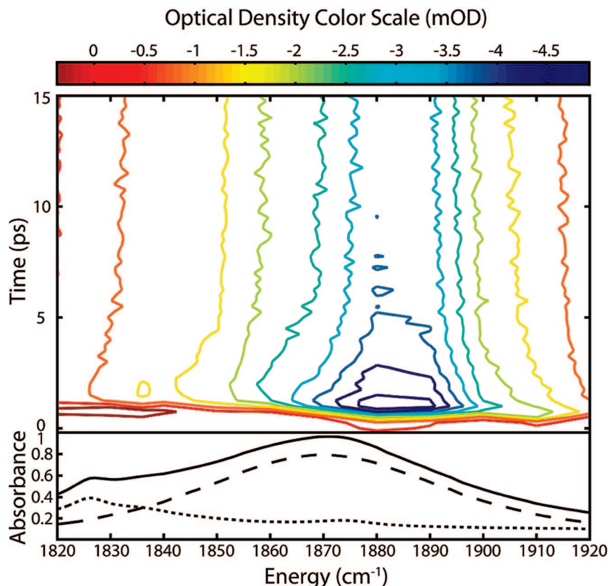
Figure 4. (Top) Contour plot of TRIR optical-density evolution observed in the NO-stretch fundamental of CINO dissolved in acetonitrile. The absolute change in optical density is indicated by the contour lines, with the color scale shown above the plot. (Bottom) The IR absorption spectra of CINO in acetonitrile (solid), acetonitrile only (short dashed), and the NO-stretch of CINO (long dash).
