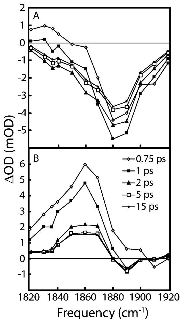
Figure 5. (A) Transient IR absorption spectrum of CINO dissolved in acetonitrile. The time delay for each spectrum is given in the figure. (B) Transient IR absorption difference spectrum. Each spectrum is the difference between the measured absorption and the predicted CINO absorption spectrum at each time delay.
