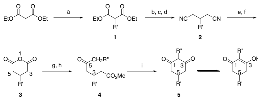
Scheme 1. Preparation of mono and 2,5-dialkylated 1,3-cyclohexanediones exhibiting diverse alkyl substituents. Reagents and conditions: (a) \text{NaOEt} , \text{R}'\text{X} (82–95%); (b) \text{LiAlH}_4 (95–98%); (c) \text{py} , \text{MsCl} (73–93%); (d) \text{KCN} (80–98%); (e) \text{aq NaOH} (75–98%); (f) \text{TFAA} (97–100%); (g) \text{Cd}(\text{CH}_2\text{R}'')_2 (78–99%); (h) \text{CH}_2\text{N}_2 (quant.); (i) \text{KO}^t\text{Bu} (73–98%).
