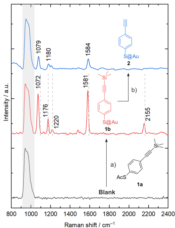
Figure 2. Immobilization of 1a on a Au nanohole array and subsequent trimethylsilyl (TMS) deprotection: SERS spectra of a blank Au nanohole array (black), TMS-protected alkyne ( 1b , red) and deprotected alkyne ( 2 , blue) SAMs on a Au nanohole array at 633 nm excitation. The Si signal of the substrate (2 nd order LO) is marked with a gray bar. The values above the signals denote the respective Raman shift in cm -1 . The spectra were separated for better visibility. The vertical dashed gray lines indicate the peak positions of the Raman spectrum of the corresponding solid. Reagents and conditions: a) Au nanohole array chip, 1a , aq. NH 3 (7 M in MeOH), EtOH, 23 °C, 24 h; b) tetrabutylammonium fluoride (TBAF), tetrahydrofuran (THF), ultrasound, 40 °C, 1 h.
