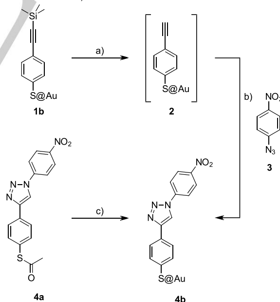
Scheme 1. Deprotection of (a) the TMS-protected alkyne of 1b with (b) the immediately following CuAAC reaction on the liberated alkyne of 2 on Au nanohole arrays, yielding triazole 4b . c) Immobilization of 4a on Au nanohole arrays. Reagents and conditions: a) TBAF, THF, ultrasound, 40 °C, 1 h; b) 1-Azido-4-nitrobenzene ( 3 ), CuSO 4 ·5 H 2 O, sodium ascorbate, THF/H 2 O, ultrasound, 40 °C, 1 h, then 23 °C, 16 h; c) Au nanohole array chip, NH 3 (7 M in MeOH), CHCl 3 , 23 °C, 5.5 h.
