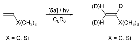
Scheme 3. H/D Exchange in Vinyltrimethylsilane and 2,2-Dimethylbutene Catalyzed by 5a
