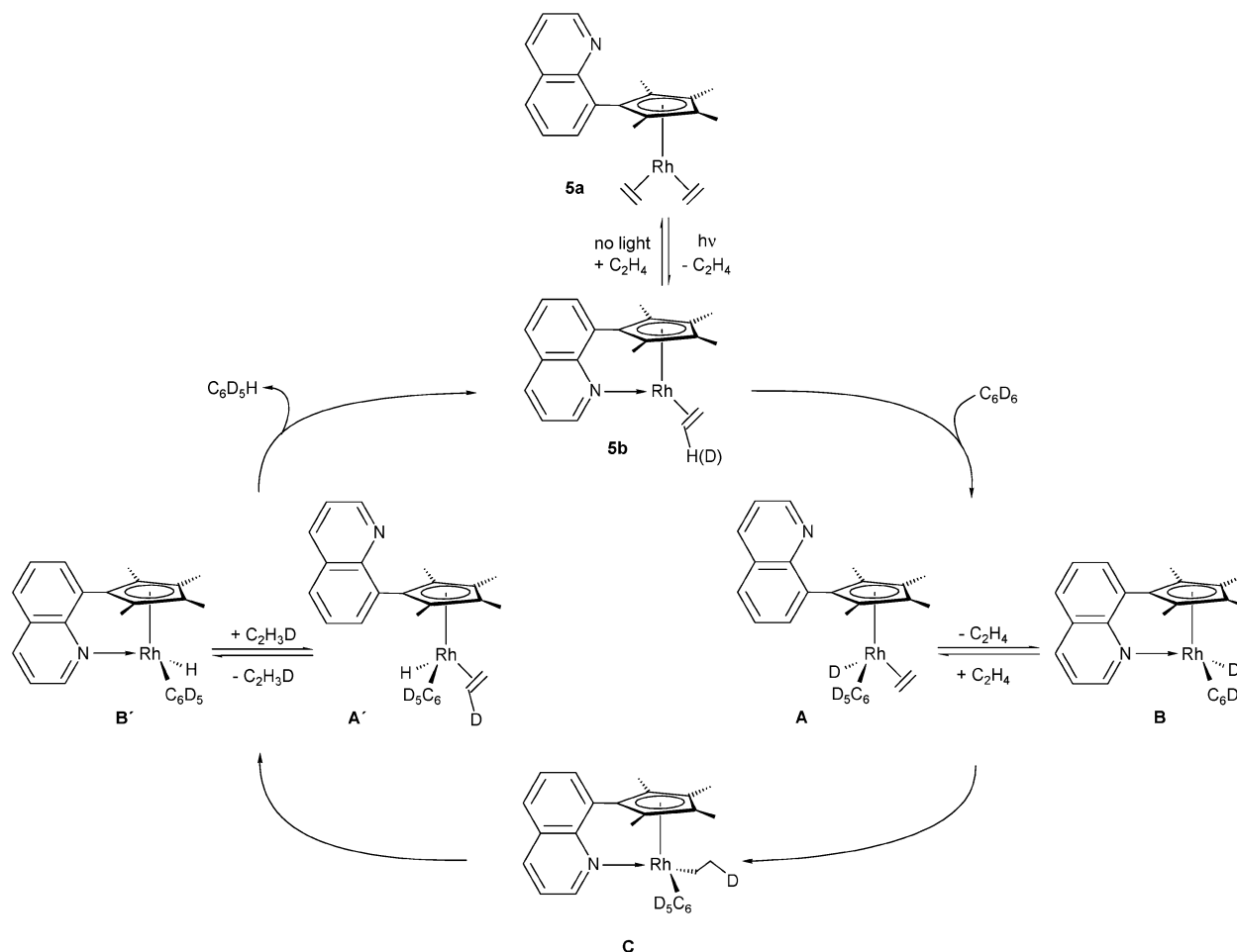
Scheme 2. Proposed Catalytic Cycle for H/D Exchange in Ethene Ligands with Complexes 5a/5b a
