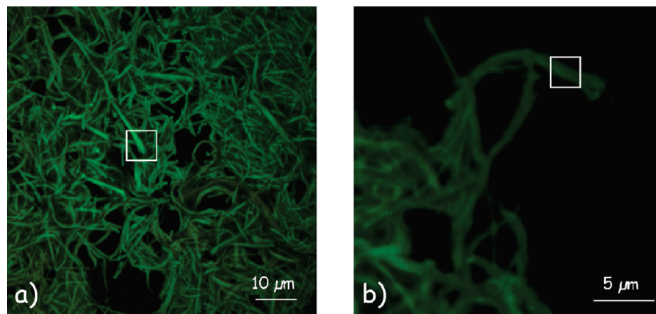
Figure 5. 80 \times 80 \mu\text{m}^2 (a) and 25 \times 25 \mu\text{m}^2 (b) LSCM images of xerogels of compound 1 in DMF deposited on a microscope coverslip. Excitation wavelength 408 nm and 60\times oil-immersion microscope objective.
