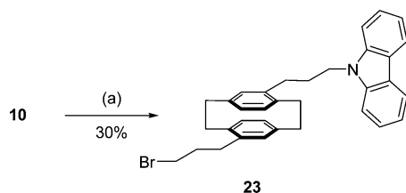
Scheme 4. Synthesis of the Reference Compounds, Cz-(CH 2 ) 3 -[2.2]PCP-(CH 2 ) 3 Br 23 a
