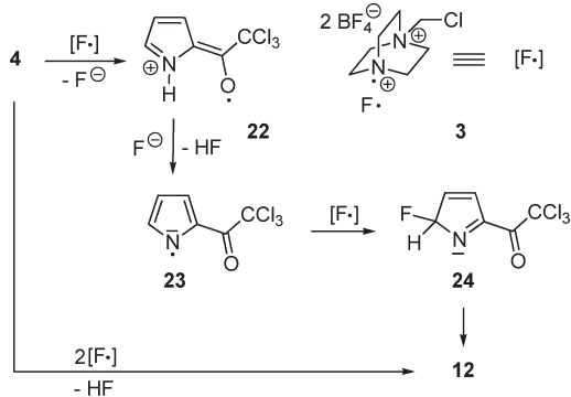
Scheme 3. Possible SET Mechanism of 5-Fluorination
