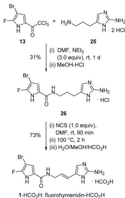
Scheme 4. Synthesis of Fluorohymenidin ( 1 ) via One-Step Dehydrogenation of Dihydrofluorohymenidin ( 26 )
