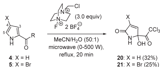
Scheme 2. Oxidation of Trichloromethylketones 4 and 5
