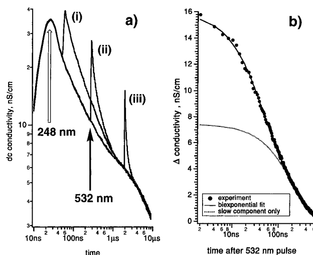
Figure 1. (a) Change in the conductivity induced by the 532 nm laser pulse (40 mJ) from a Nd:YAG laser in two-color photolysis of 8 \times 10^{-6} \text{ mol dm}^{-3} triphenylene in \text{CO}_2 -saturated cyclohexane. A 20 ns pulse (248 nm, 30 mJ) occurred at time shown by a broad arrow; the 532 nm pulse was applied after (i) 30 ns, (ii) 270 ns (shown by an arrow), and (iii) 2 \mu\text{s} . The change in the conductivity is due to formation of HMI by photoexcitation of the triphenylene radical cation. (b) Trace iii from (a); the conductivity induced by the 248 nm pulse is subtracted. The difference trace (the decay kinetics of HMI) is fit by a sum of two exponentials. The slow component with a lifetime of 260 ns is given by the broken line; the fast component has a lifetime of 30 ns.
