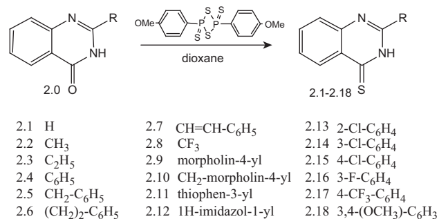
Scheme 3. Synthesis of 2-R-quinazolin-4(3H)-thiones.
