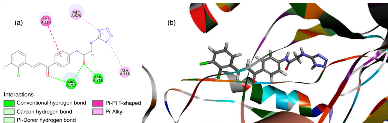
Fig. 1. 2D (a) and 3D (b) model of compound 34 docked with 1T9U protein
