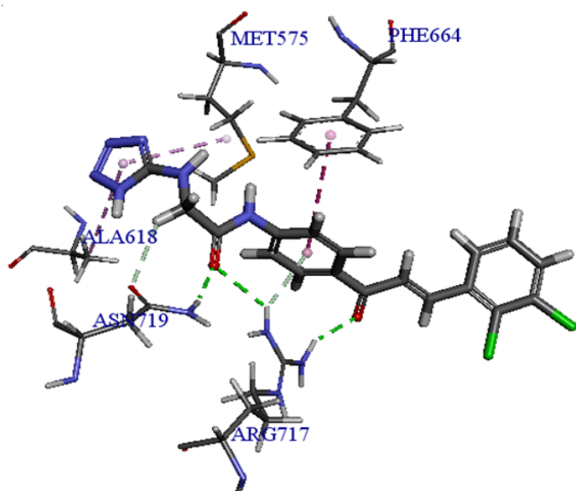
Fig. 2. Docking interactions of 1T9U protein with compound 34
