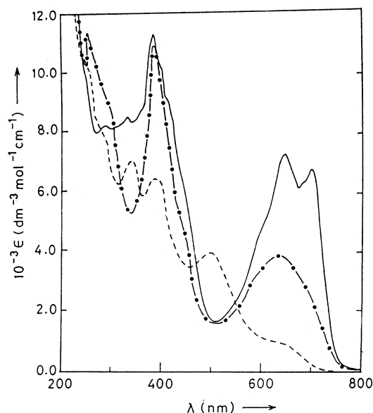
Fig. 3. UV-vis spectra of \text{Pd}(\text{NaiCH}_2\text{Ph})\text{Cl}_2 ( 3c ) (---), \text{Pd}(\text{NaiCH}_2\text{Ph-H})\text{Cl} ( 4c ) (-●-●-) and \text{Pd}(\text{NaiCH}_2\text{PhO})\text{Cl} ( 5c ) (—) in MeCN at 298 K.
