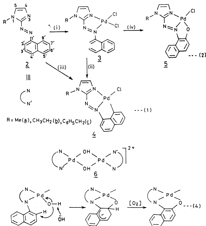
Scheme 1. (i) PdCl 2 in MeCN/Na 2 [PdCl] in MeOH, stir; (ii) CH 2 Cl 2 –MeOH, NaOAc, pH 4.5–6.0, stir; (iii) Pd(OAc) 2 in C 6 H 6 , reflux; and (iv) NaOH in MeCN/AgOH, stir or AgNO 3 reflux.
