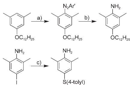
Scheme 1. Synthesis of the new anilines. a) AcOH, 2,4-(NO 2 ) 2 C 6 H 3 N 2 + Cl - , 0°C; b) H 2 , Pd/C, THF/MeOH; c) 1,4-C 6 H 4 (CH 3 )(SH), i PrOH, HOC 2 H 4 OH, CuI, K 2 CO 3 , 80°C.
