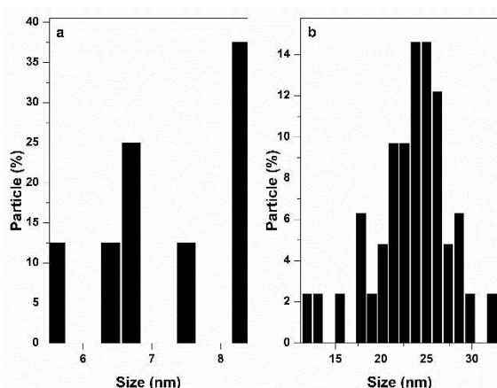
Figure 5. Particle size distribution samples IAICu15 (a), SAICu15 (b).
