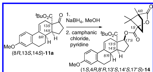
Scheme 3. Determination of the Absolute Configuration of 11a
