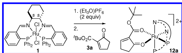
Scheme 4. Dicationic Adduct 12a of \beta -Ketoester 3a
