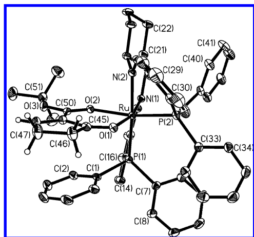
Figure 1. ORTEP drawing of 12a . Selected distances ( \text{\AA} ): Ru–P(1) 2.2973(8), Ru–P(2) 2.2692(8), Ru–N(1) 2.047(3), Ru–N(2) 2.083(3), Ru–O(1) 2.107(2), Ru–O(2) 2.172(2), C(48)–C(49) 1.339(5) \text{\AA} .
