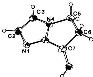
Figure 1. Molecular Structure of 1
