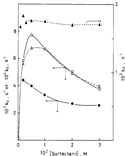
Figure 3. Effect of surfactant concentration on the rate constants at pH 7.30, 0.02 M phosphate buffer, and 25 °C: [ 1b ] = 1.00 \times 10^{-3} M; [PNPA] = 1.0 \times 10^{-4} M; (O, Δ) acylation rate constants in the presence of 2a and 2b ; (●, ▲) deacylation rate constants in the presence of 2a and 2b .
