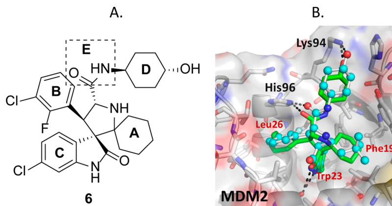
Figure 2. (A) Chemical structure of compound 6 and five regions (A–E) where chemical modifications were made. (B) Cocystal structure of 2 (light blue spheres, PDB code 5TRF) and model of the binding mode of 6 (green sticks) in complex with MDM2.
