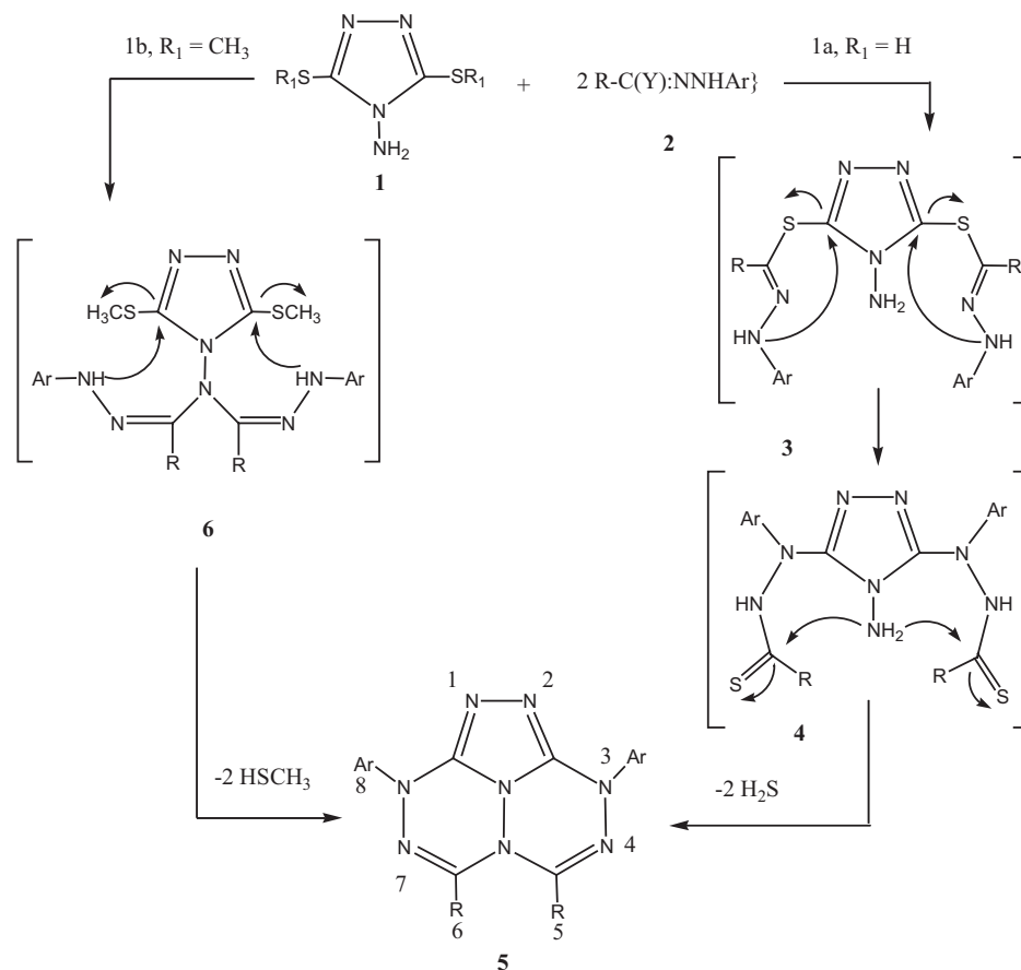
Scheme 1 Synthesis of 1,2,3,4,5a,7,8,8b-octaaza-acenaphthylenes.
