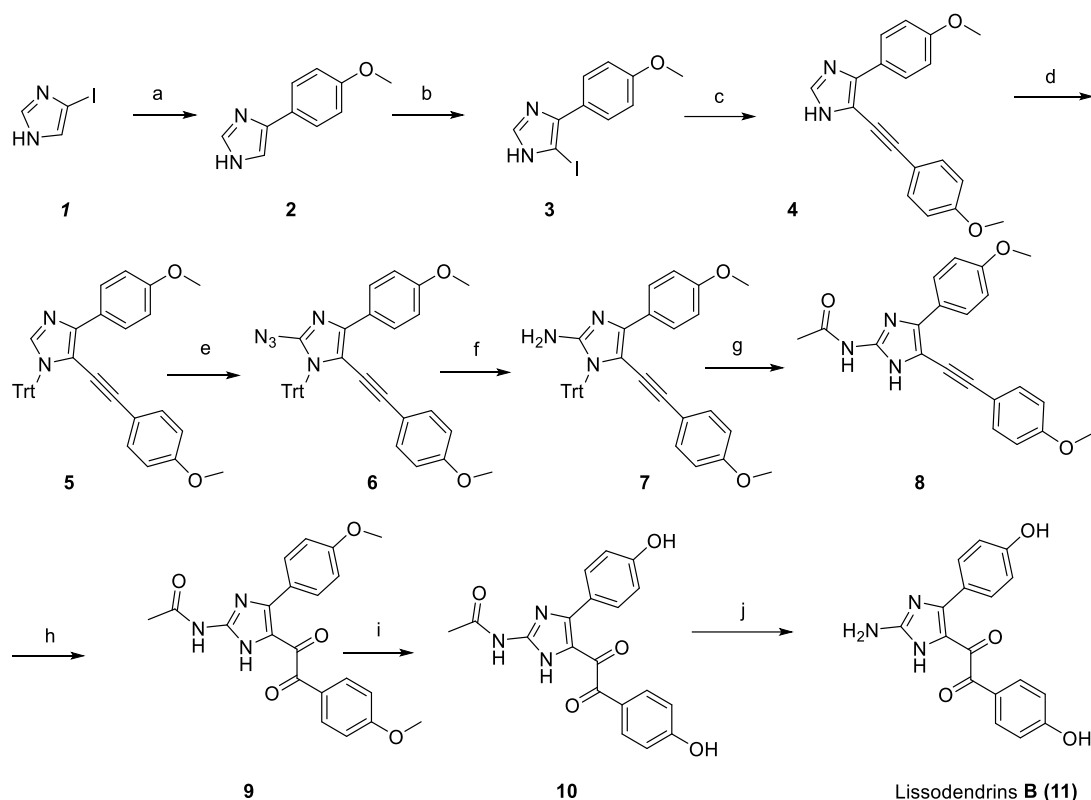
Scheme 2. Synthesis of Lissodendrin B. Reagent and conditions: (a) 4-methoxyphenylboronic acid, \text{Pd}(\text{PPh}_3)_4 , CsF, toluene, \text{H}_2\text{O} , 100^\circ\text{C} , 24 h, 82%; (b) NIS, \text{CH}_2\text{Cl}_2 , r.t., 4 h, 79%; (c) 4-methoxyphenylacetylene, \text{Pd}(\text{PPh}_3)_4 , CuI, TEA, DMF, 80^\circ\text{C} , 8 h, 70%; (d) \text{Ph}_3\text{CCl} , TEA, \text{CH}_2\text{Cl}_2 , reflux, 4 h, 77%; (e) n\text{-C}_4\text{H}_9\text{Li} , \text{TsN}_3 , THF, -78^\circ\text{C} , 6 h, 46%; (f) \text{Na}_2\text{S}\cdot 9\text{H}_2\text{O} , \text{CH}_3\text{OH} , r.t., 4 h, 69%; (g) 1) \text{Ac}_2\text{O} , TEA, \text{CH}_2\text{Cl}_2 , reflux, 4 h; 2) \text{HCl} , \text{CH}_3\text{OH} , r.t., 4 h, 62%; (h) \text{Hg}(\text{NO}_3)_2 , DMF, r.t., 4 h, 51%; (i) \text{BBr}_3 , \text{CH}_2\text{Cl}_2 , r.t., 4 h, 66%; (j) concentrated \text{H}_2\text{SO}_4 , \text{CH}_3\text{OH} , \text{H}_2\text{O} , reflux, 4 h, 51%.
