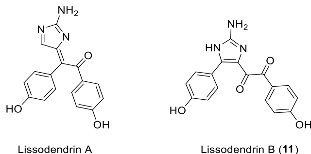
Figure 1. Structures of Lissodendrin A and Lissodendrin B.
