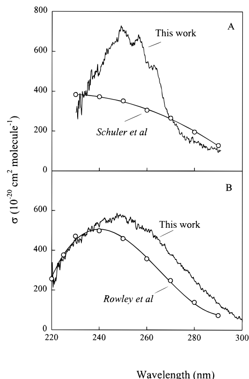
Figure 2. (A) UV-absorption spectrum of the c-C 6 H 11 • radical reported by Schuler and Patterson 6 (circles) and measured herein (solid line). (B) UV-absorption spectrum of the (c-C 6 H 11 )O 2 • radical reported by Rowley et al. 13 (circles) and measured in the present work (solid line).
