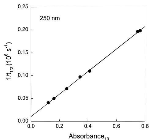
Figure 3. Plot of the reciprocal half-life for self-reaction of c-C 6 H 11 • radicals as a function of the maximum absorbance at 250 nm.
