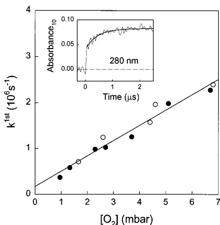
Figure 4. Pseudo-first-order rate constants for the formation of (\text{c-C}_6\text{H}_{11})\text{O}_2^\bullet radicals as a function of the \text{O}_2 concentration in 500 (opened circles) and 1000 (filled circles) mbar of \text{SF}_6 , diluent. The insert shows an experimental transient obtained using a mixture of 5 mbar \text{c-C}_6\text{H}_{12} , 5.1 mbar \text{O}_2 , and 990 mbar \text{SF}_6 . The UV path length was 80 cm and the radiolysis dose was 32% of maximum. The smooth curve in the insert is the first-order fit (starting at t = 0.2 \mu\text{s} ).
