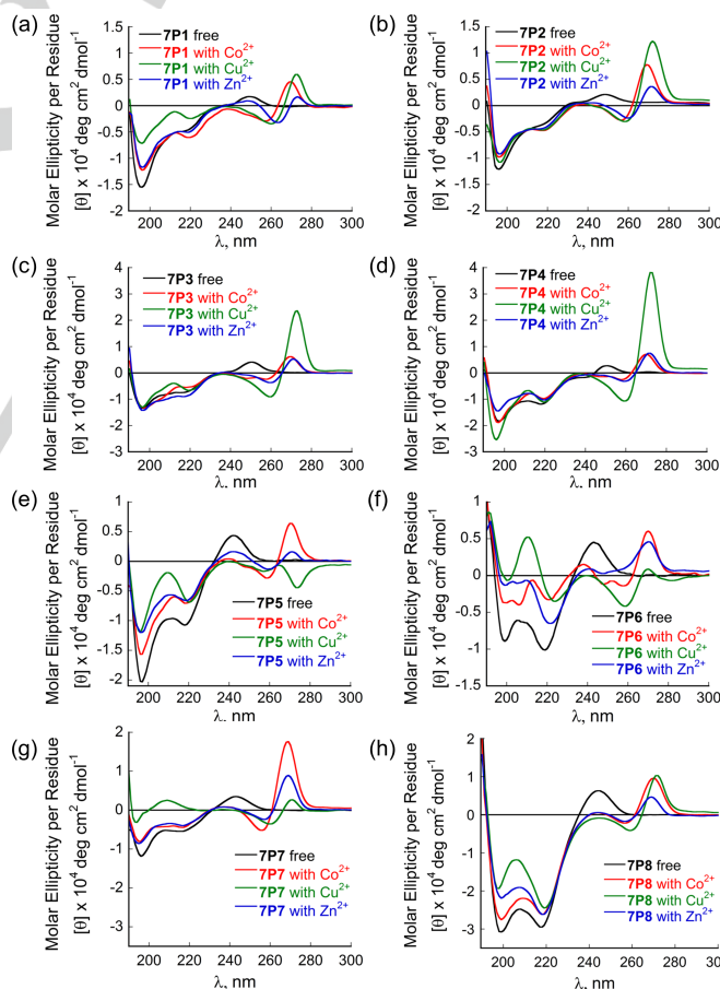
Figure 3. CD spectra of oligomers 7P1-7P8 and their \text{Co}^{2+} , \text{Cu}^{2+} , \text{Zn}^{2+} complexes (100 \mu\text{M} in 80% aqueous methanol).
