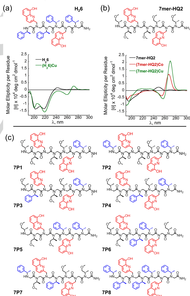
Figure 1. (a) Chemical sequence of H 2 .6 and CD spectra of H 2 .6 and its Cu 2+ complex. 6 (b) Chemical sequence of 7mer-HQ2 and CD spectra 7mer-HQ2 and its metal complexes. 7 (c) Chemical sequences of oligomers 7P1–7P8 .
