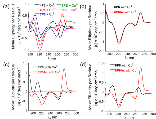
Figure 7. CD spectra of (100 μM in 80% aqueous methanol): (a) Cu 2+ complexes of 4P6 , 6P6 , 7P6 , 7P6I , 8P6 . (b) Cu 2+ complexes of 6P6 and 6P6Ac (c) Cu 2+ complexes of 7P6 and 7P6Ac (d) Cu 2+ complexes of 8P6 and 8P6Ac .
