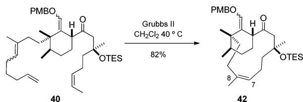
Scheme 7. RRCM of 40
