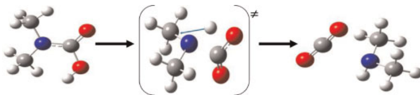
Figure 3. Decarboxylation reaction of the unstable N-substituted carbamic acids. The TS structure is a four-membered ring (N—C—O—H) and the imaginary frequency is associated with the hydrogen transfer. This figure is available in colour online at www.interscience.wiley.com/journal/poc
