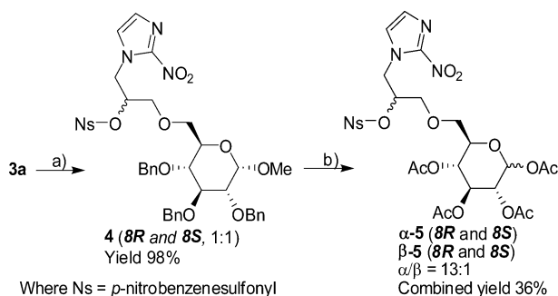
Scheme 3. Preparation of Compound 5, a Useful Intermediate for Synthesizing F-18 Labeled 11 a
