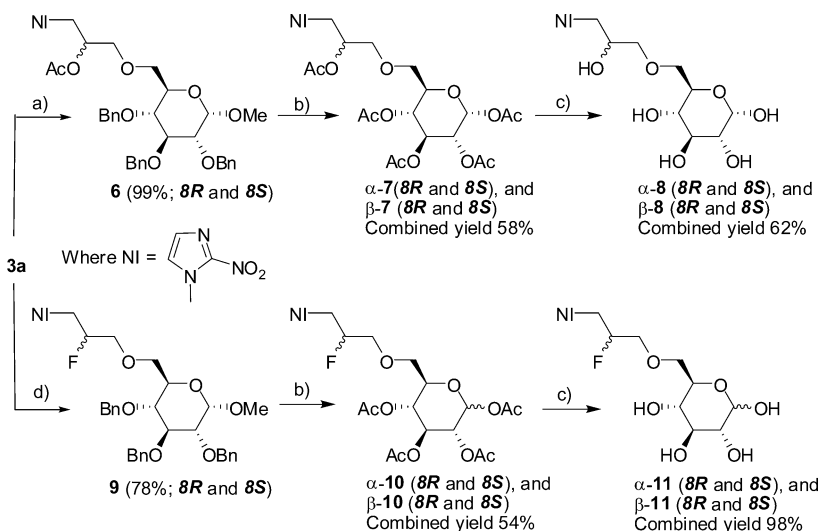
Scheme 2. Preparation of Compounds 8 and 11 a
