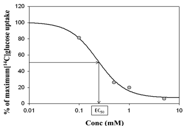
Figure 5. Estimation of the median effective concentration ( EC_{50} ) for the inhibition of [ 14 C]glucose uptake by uptake by oocytes expressing GLUT-2 in the presence of 13.
