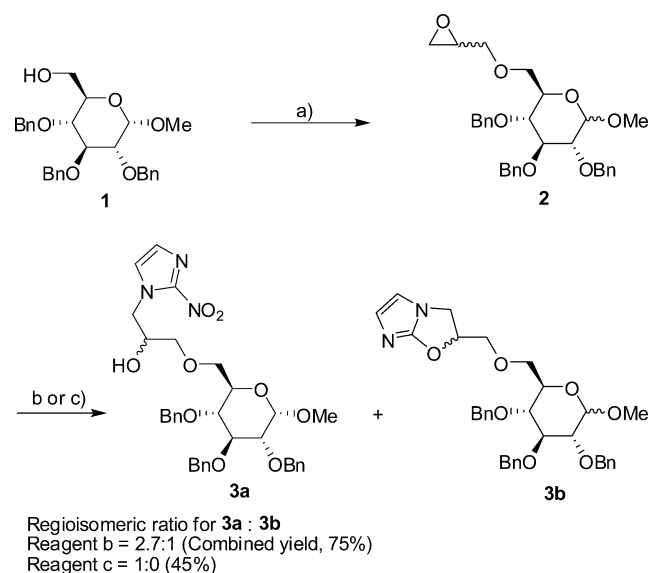
Scheme 1. Preparation of Glucose-6- O -Linked Azomycin Conjugates a
