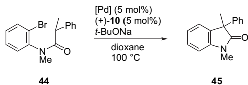
Scheme 7. Palladium-catalyzed intramolecular \alpha -arylation.
