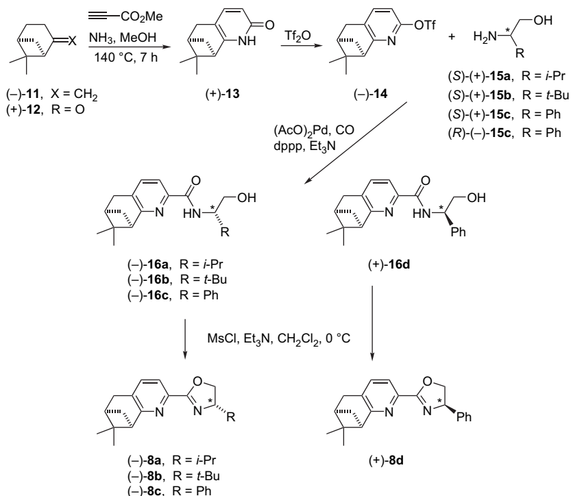
Scheme 1. Synthesis of pyridyl oxazoline ligands from \beta -pinene.
