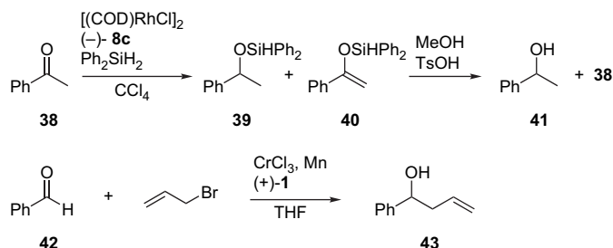
Scheme 6. Rhodium-catalyzed hydrosilylation and Nozaki–Hiyama–Kishi allylation.
