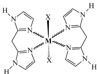
Structure of \text{Cu}(\text{BIM})_2\text{Cl}_2
