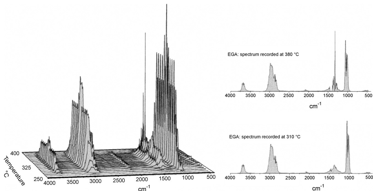
Fig. 2. Infrared spectra of the TG evolved gases for the decomposition of \text{M}(\text{BIM})_2\text{Cl}_2 complexes in the temperature range 250–400 °C. Air flow at 100 mL min −1 rate. Resolution: 8 cm −1 , 10 scans per spectrum.
