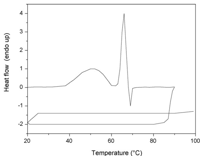
Fig. 3. DSC curve of the \text{Co}(\text{BIM})_2\text{Cl}_2 . Closed pan. Scanning rate: 10^\circ\text{C min}^{-1} .
