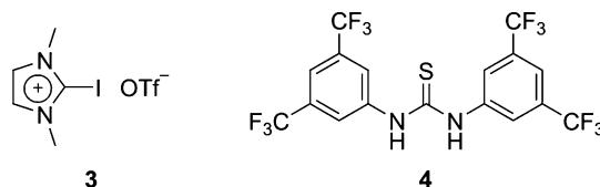
Figure 3. Imidazolium derivative 3 and thiourea 4, tested for comparison with the bidentate XB donors.
