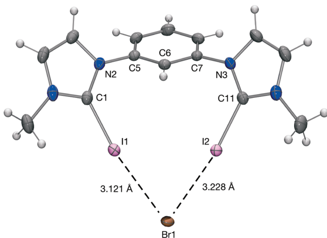
Figure 2. X-ray structural analysis of the complex of bromide with m -II-1 Me /BPh 4 (anion omitted for clarity; ellipsoids at 50% probability). Selected bond lengths [Å] and angles [°]: C1–I1 2.090, C11–I2 2.083, C11–I2–Br1 170.5, C1–I1–Br1 172.1, C11–N3–C7–C6 54.4, C6–C5–N2–C1 –60.0.
