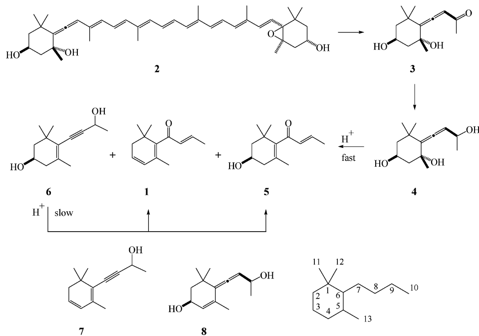
Figure 1. Proposed pathway for the formation of 1 from neoxanthin (2), including the structures of two tentatively identified intermediates, 7 and 8, and the generic numbering scheme employed for megastigmane derivatives (5).
