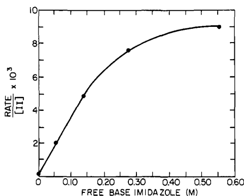
Figure 3. Plot of the hydrolysis rate/[II] vs. the molar concentration of free base imidazole in a pH 7.1 buffer. From (\text{rate})/[\text{II}] = k_1 + k_2[\text{Im}]^n , the initial linearity where [\text{Im}] < 0.30 M indicates that n = 1 : k_1 = y intercept and k_2 = \text{slope} for the linear section of the curve.
