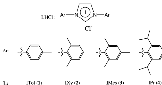
Scheme 1. Imidazolium Salts
