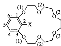
[Formula of (2-X-1,3-phenylene)-19-crown-6]
