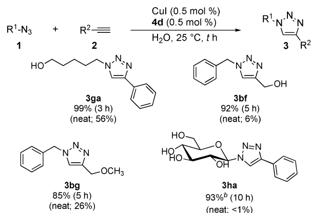
Scheme 1. CuAAC Reaction in the Presence of Water a
