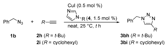
Scheme 3. CuAAC Reaction of Acetylenes with Bulky Substituents
