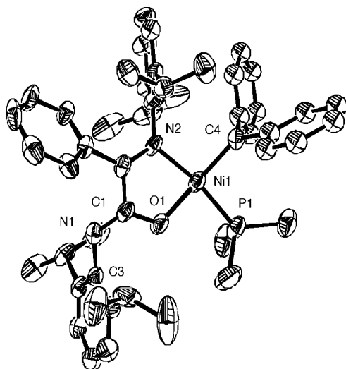
Figure 6. ORTEP drawing of 5 (R = Ph) at the 50% probability level showing both orientations of the phenyl ring on the benzyl ligand. Hydrogen atoms are omitted for clarity.
