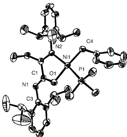
Figure 3. ORTEP drawing of 2 (R = Et) at the 50% probability level. Hydrogen atoms are omitted for clarity.
