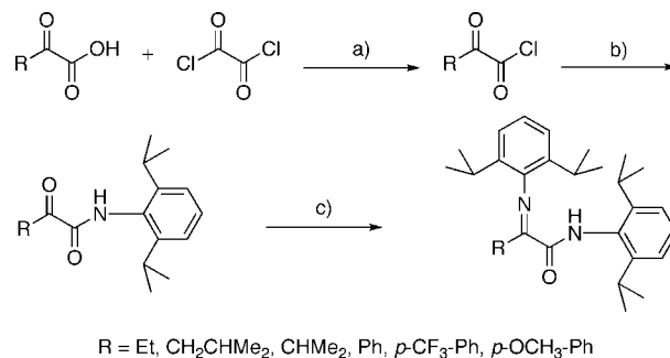
Scheme 1. Synthetic Approach to Substituted \alpha -Iminocarboxamide Ligands a
