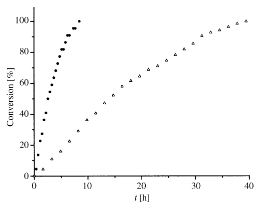
Figure 6. Curve of conversion of benzene hydrogenation catalyzed by (left) \text{Ir}^0 and (right) \text{Rh}^0 nanoparticles prepared in situ in \text{BMI} \cdot \text{PF}_6 (1 mL) at 75 °C and 4 atm (constant pressure). [M]/[substrate] ratio 1:500 (1200 rpm).
