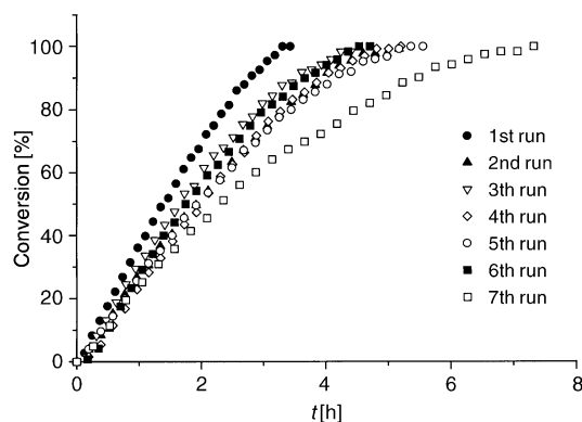
Figure 5. Conversion curves of benzene hydrogenation by \text{Ir}^0 nanoparticles "solventless" at 4 atm and 75 °C, [benzene]/[Ir] = 250, showing the catalyst recycle.
