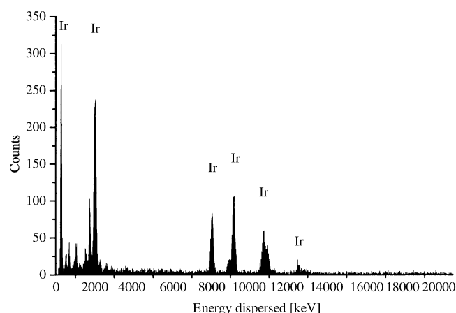
Figure 8. EDS of the Ir 0 nanoparticles prepared in BMI·PF 6 , 75 °C, H 2 (4 atm), 10 min.
